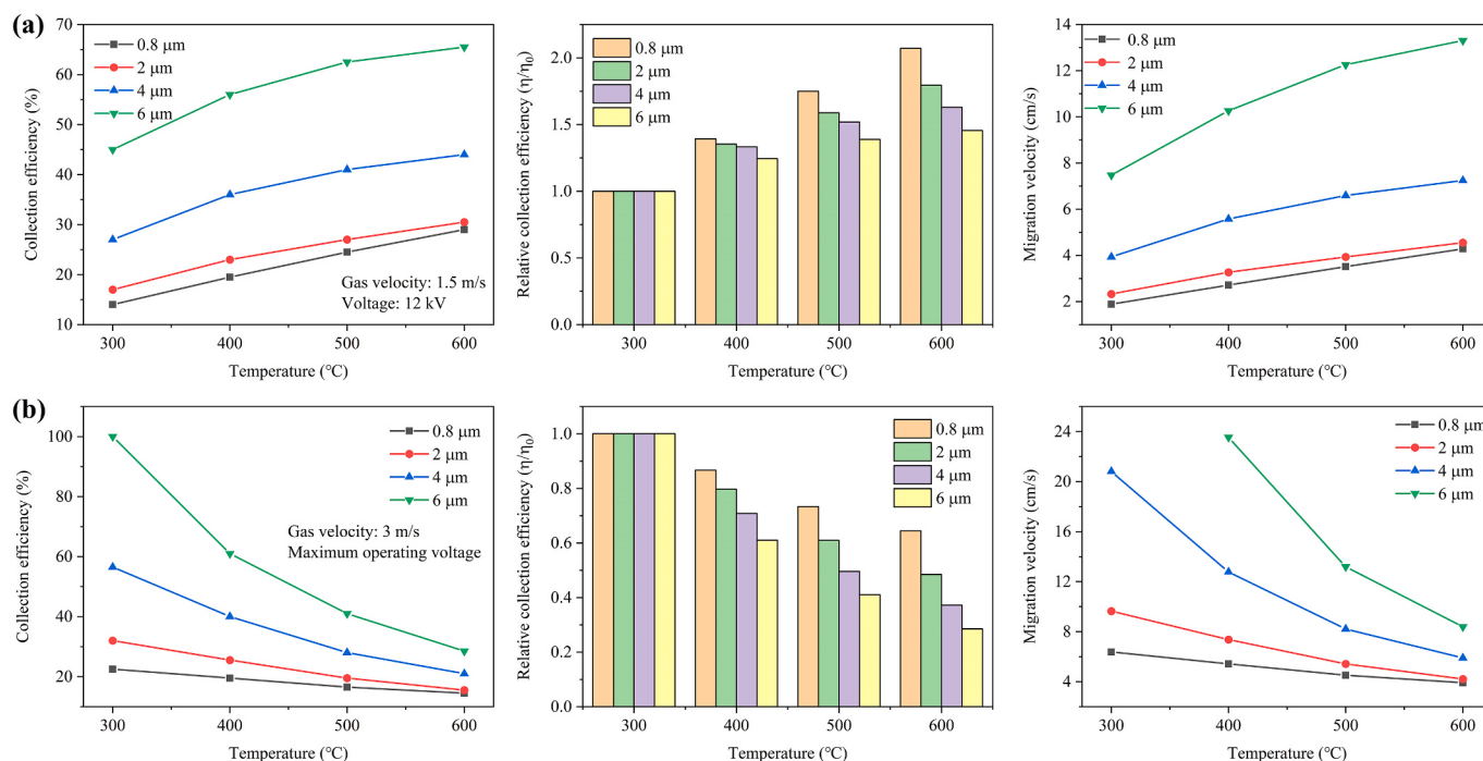
Fig. 14. Collection efficiency and migration velocity for particles with diameters of 0.8, 2, 4, 6 μm at different temperatures under (a) the same voltage (12 kV) and (b) maximum operating voltage.
